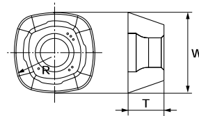
Insert with Chip Breaker
